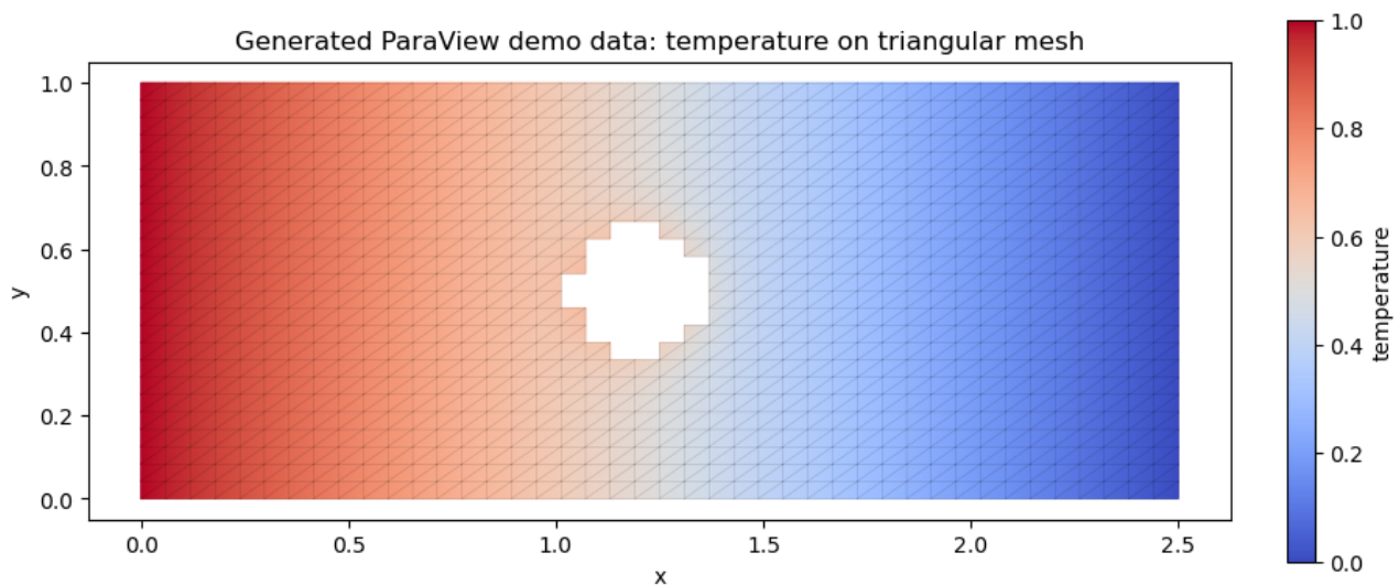
Figure 1: Generated demo data for the ParaView workflow: temperature on a triangular mesh written to VTK.
