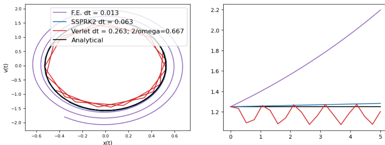
Figure 8.3.: Harmonic oscillator phase space (left) and energy (right), \omega=3
